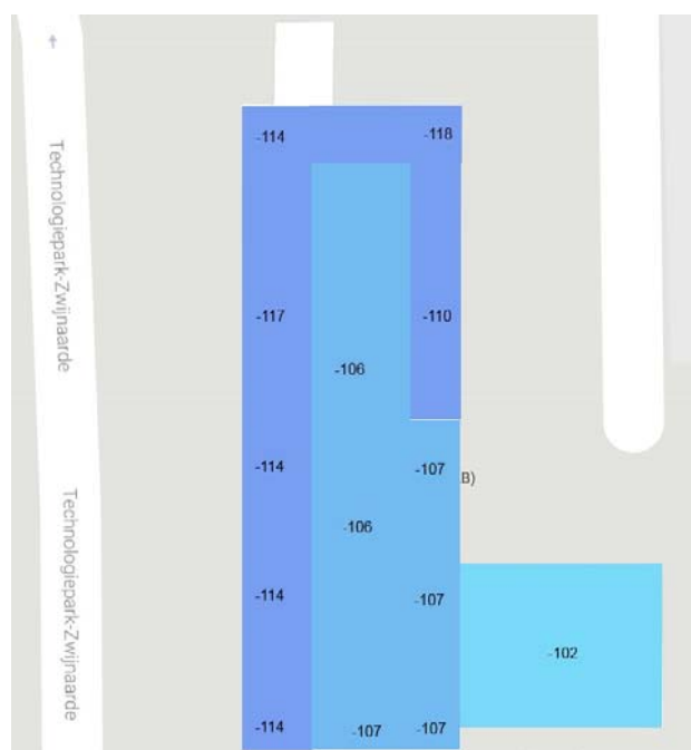
Figure 3: LoraWAN coverage of the basement floor of a campus building
