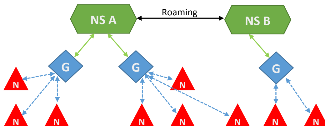
Figure 1. LoraWAN network topology
